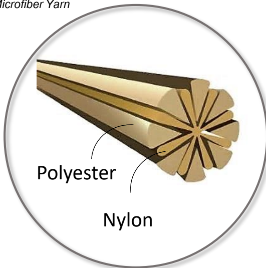
Cross Section of Microfiber Yarn
